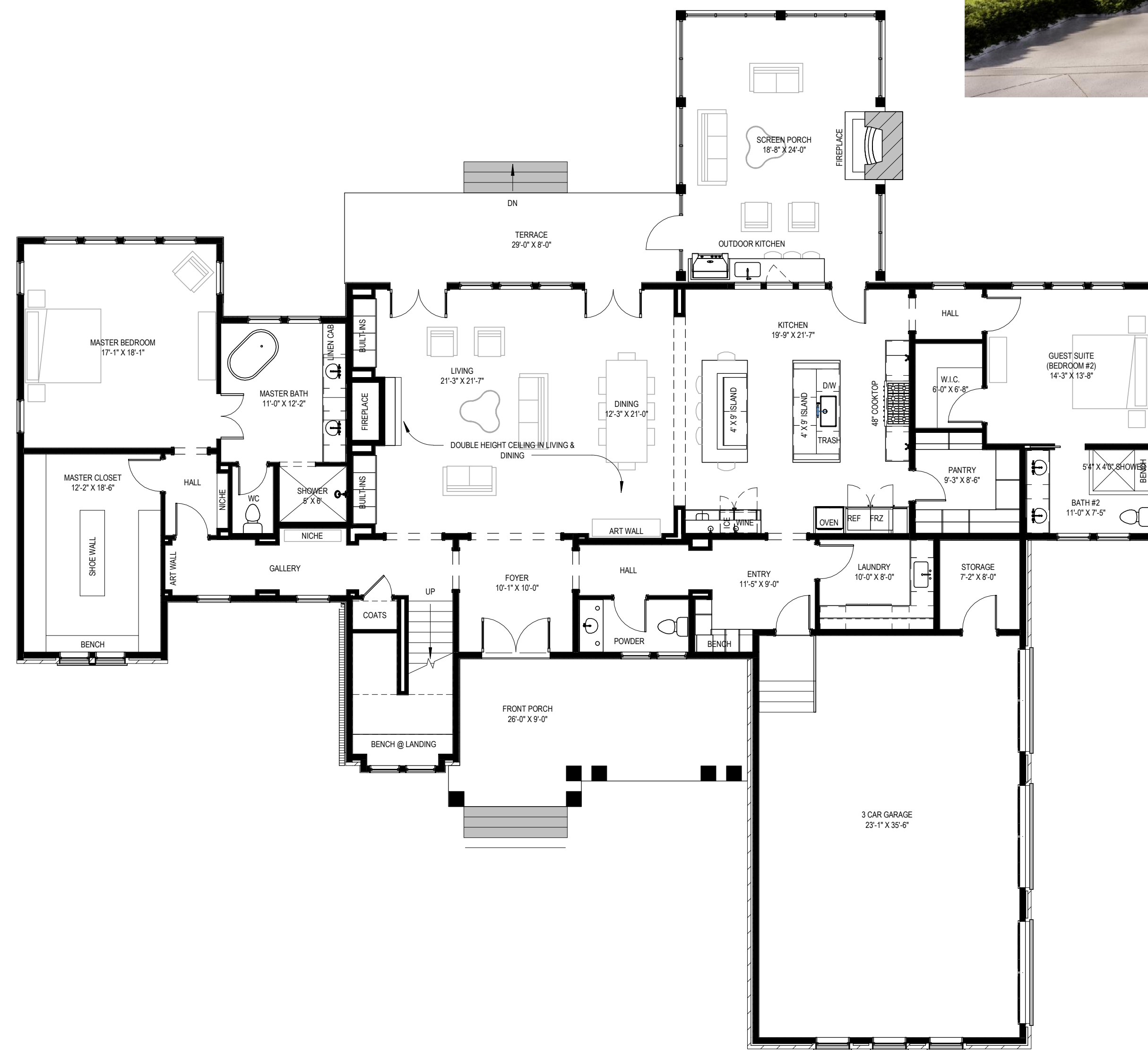
1ST FLOOR
