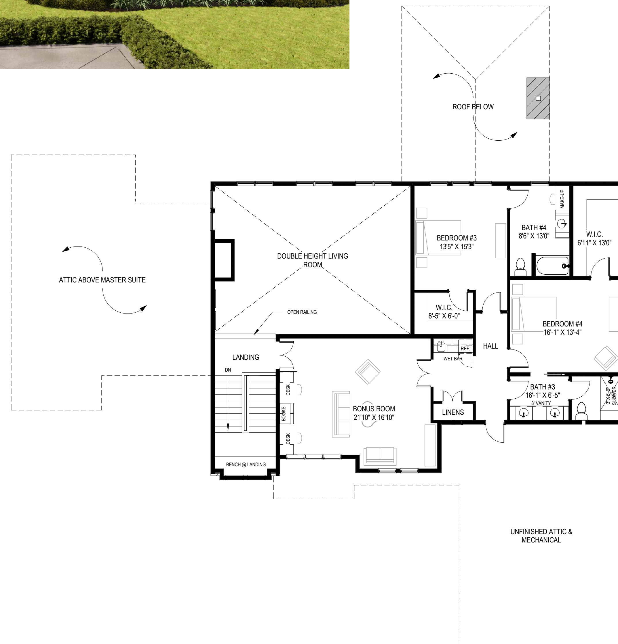
2ND FLOOR
